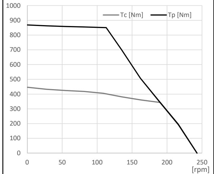
WATER COOLING
