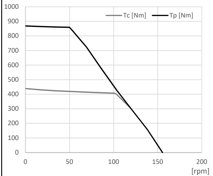
WATER COOLING
